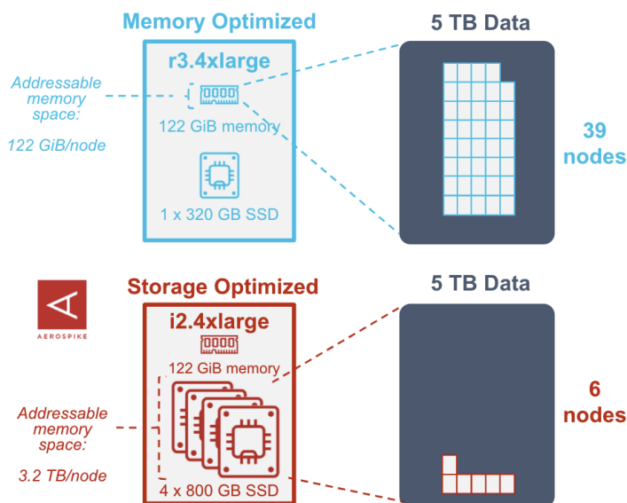
Fig. 2: Legacy architecture compared to Aerospike's HMA.
